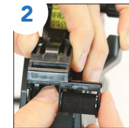
While supporting the ink roller assembly with one hand, gently slide the ink roller off to the side.
