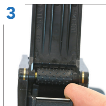
After opening the door, gently lift the pressure plate and pull to open up the entire tool.
