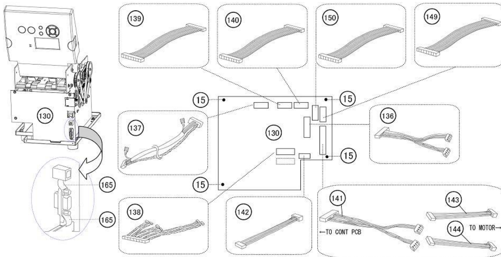
DESCRIPTION Fig09-ASSY
