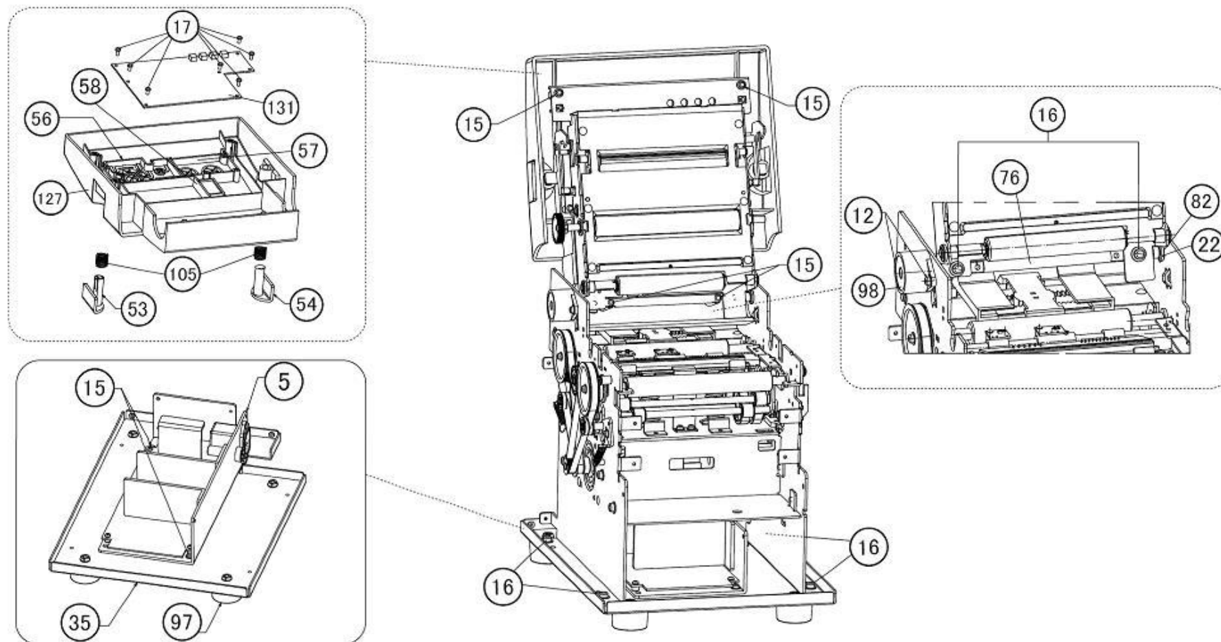
DESCRIPTION Fig07-ASSY
