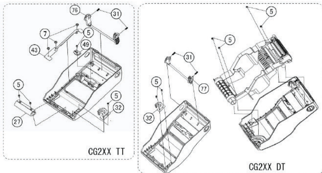
Fig PL5a, Top Cover Assembly
