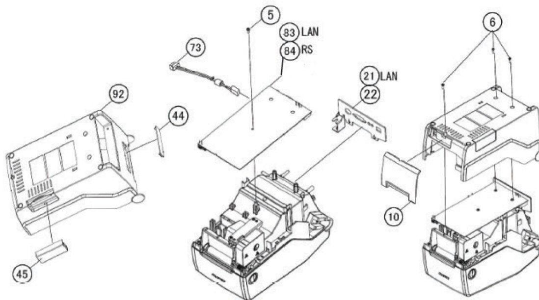
Fig PL4a, Bottom Assembly
