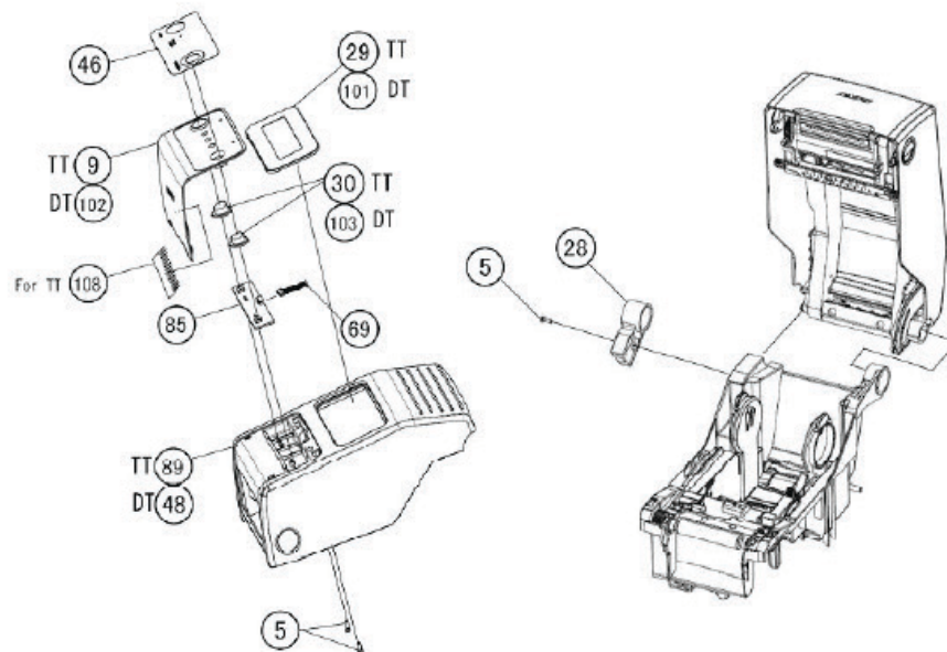
Fig PL5b, Top Cover Assembly
