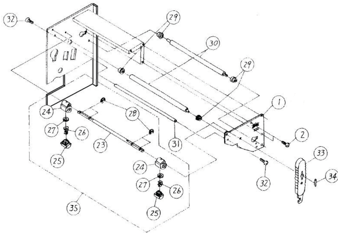
Figure PL3a, Head Assembly (1)
