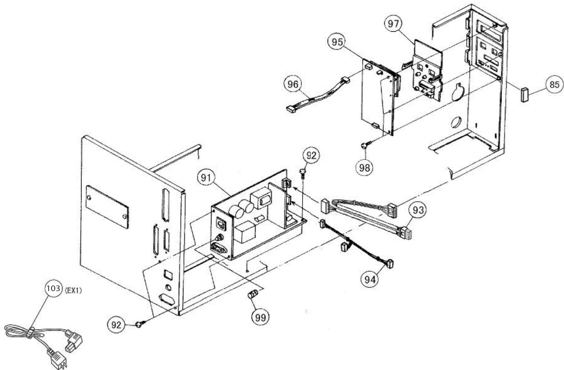
Figure PL1d, Base Cover Assembly (4)
