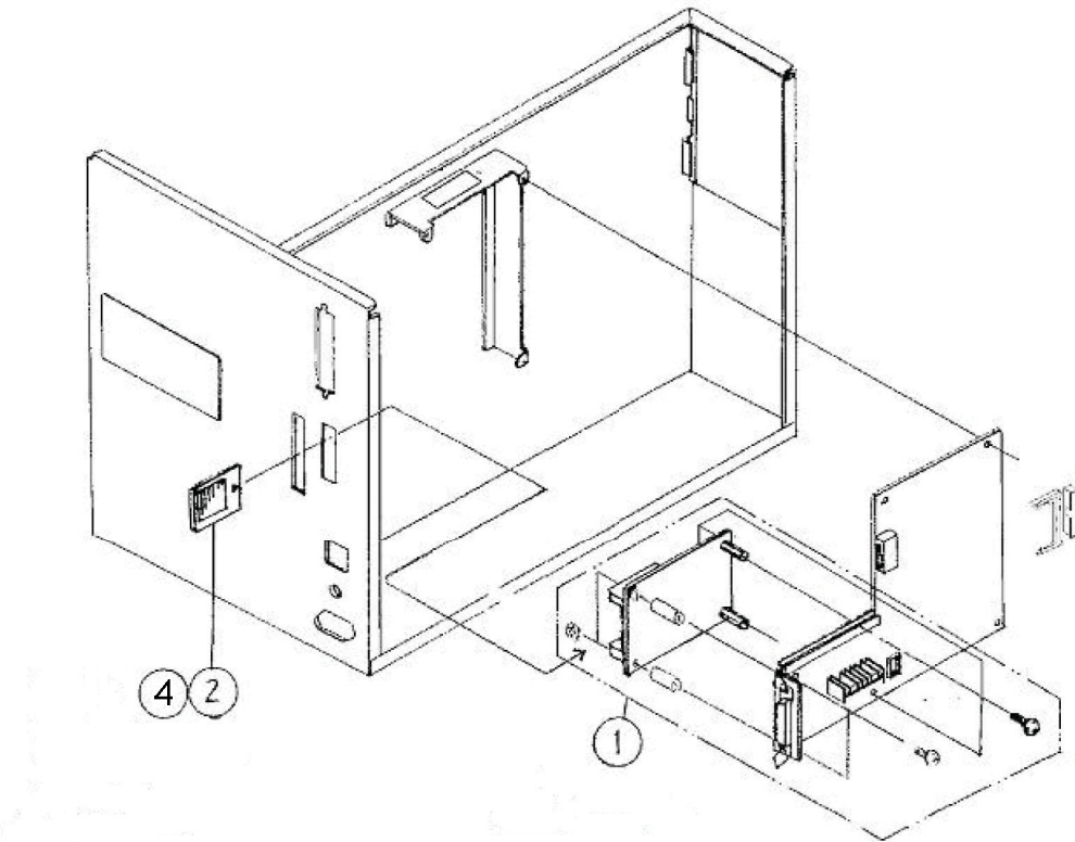
Figure PL6, PCMCIA Card Assembly
