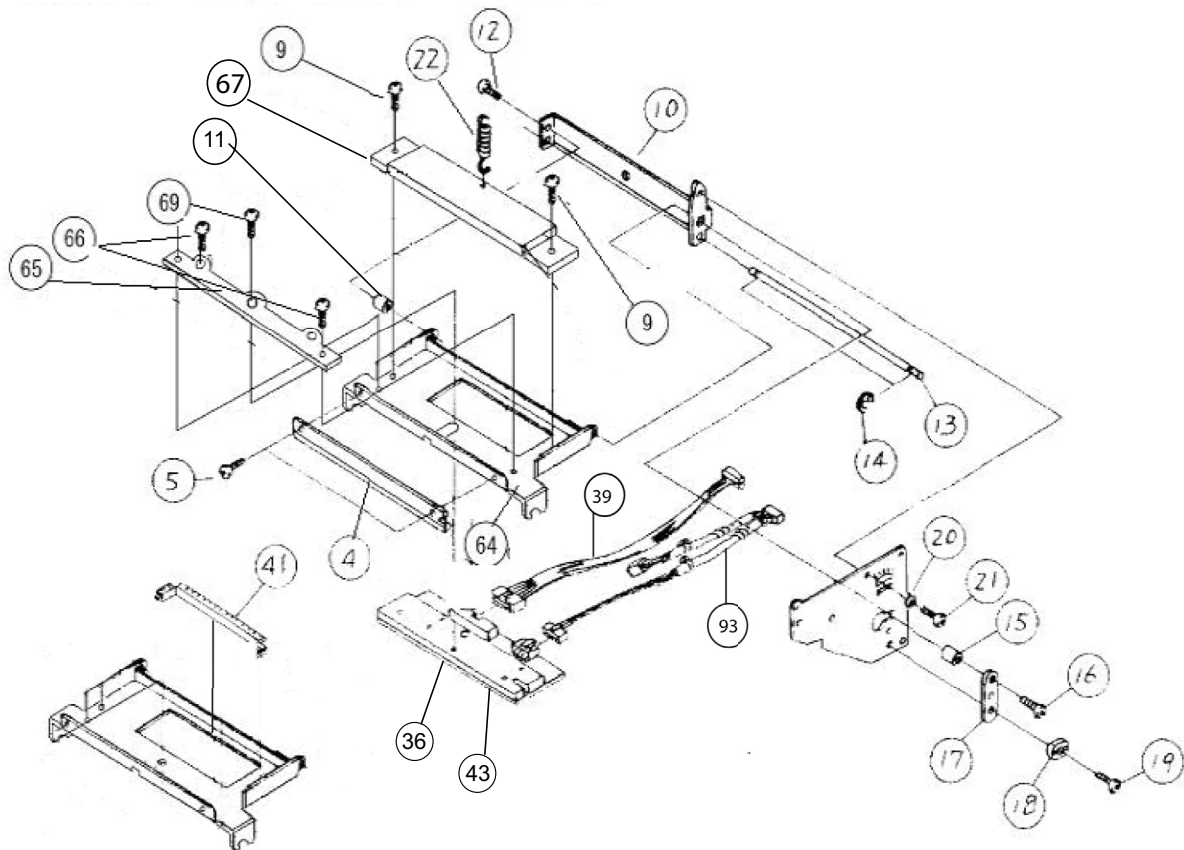
Figure PL3b, Head Assembly (2)
