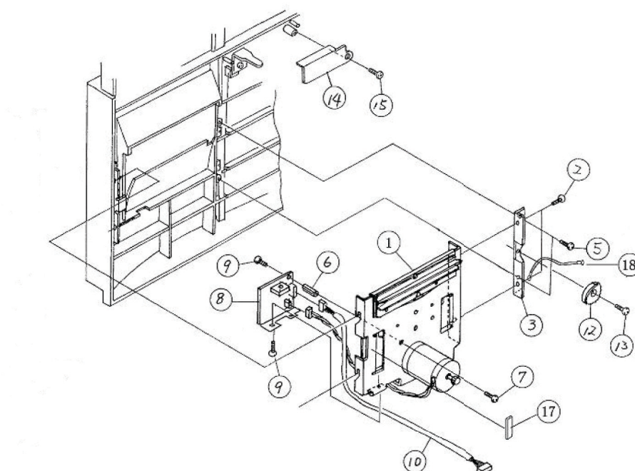
Figure PL8, Cutter Assembly
