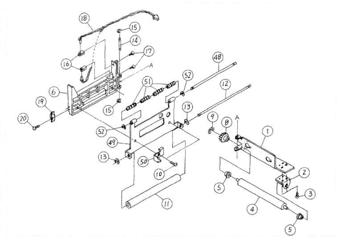
Figure PL7a, Dispense Assembly (1)
