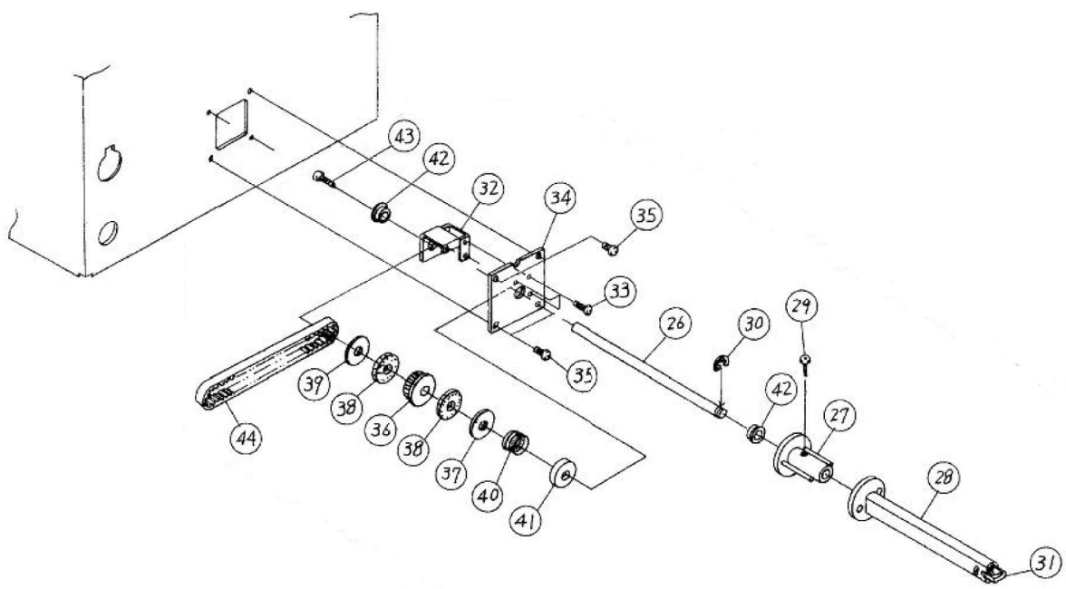
Figure PL7b, Dispense Assembly (2)
