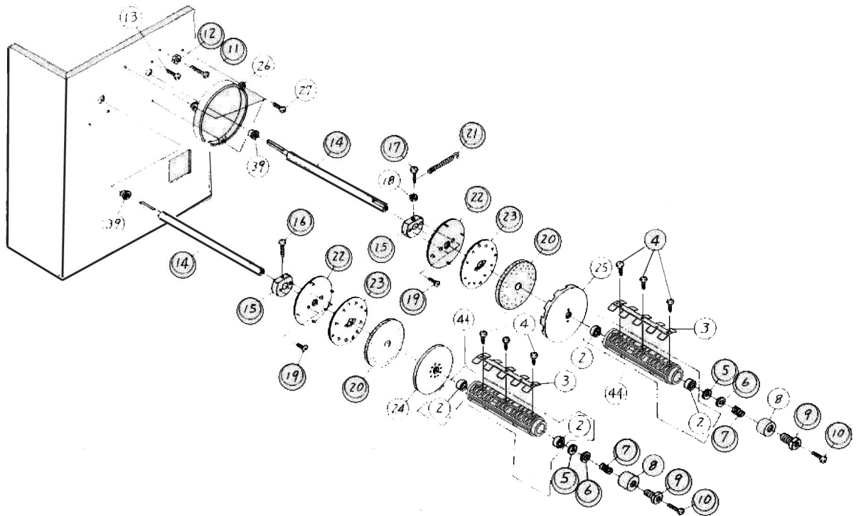
Figure PL4a, Ribbon Assembly (1)
