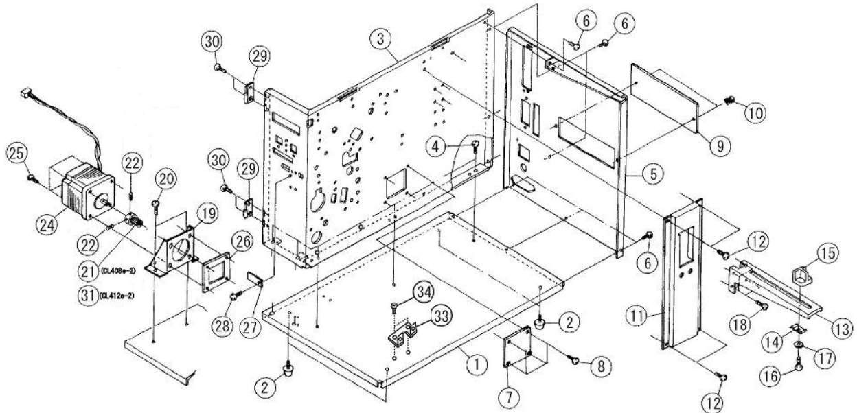
Figure PL1a, Base Cover Assembly (1)
