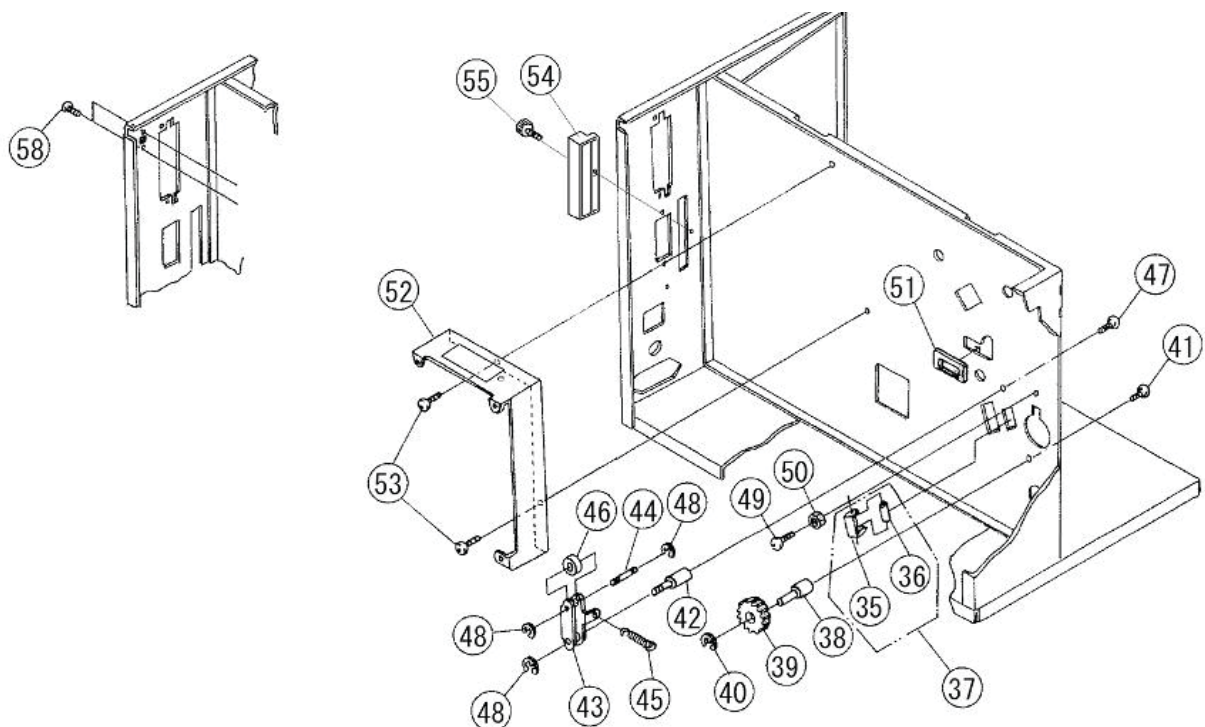
Figure PL1b, Base Cover Assembly (2)
