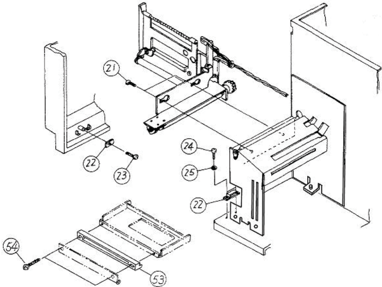
Figure PL7c, Dispense Assembly (3)
