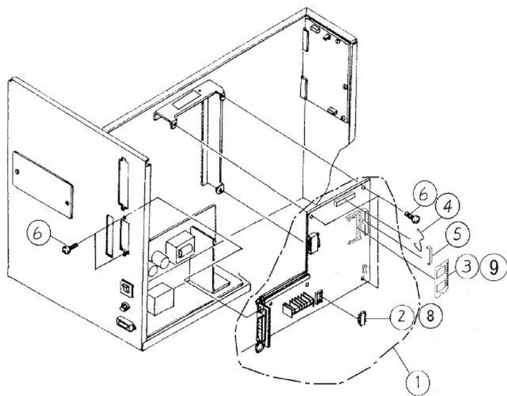
Figure PL5, PCB Assembly
