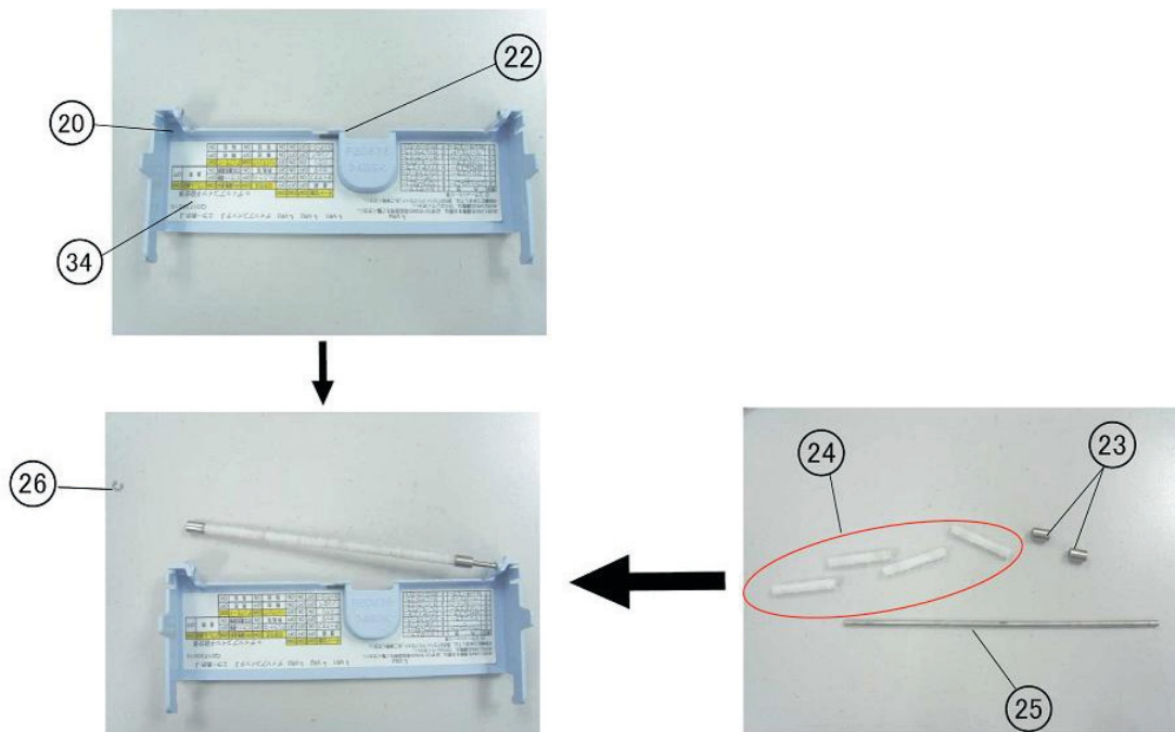
Figure PL1a, Dispense Assembly
