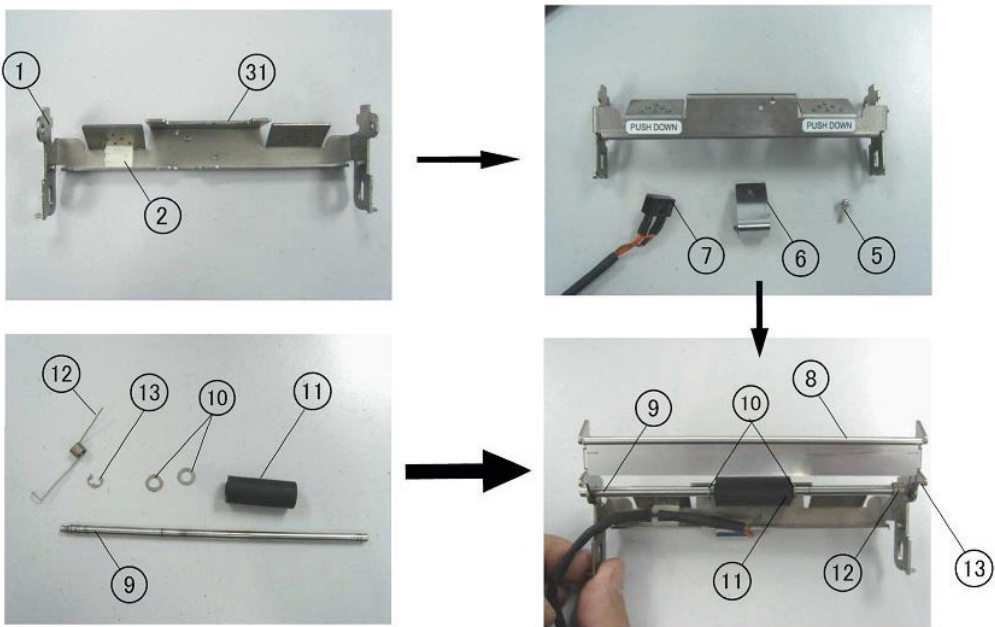
Figure PL2a, Dispense Assembly
