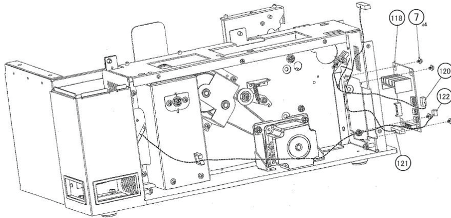
Figure PL7, PCB Cable Assembly
