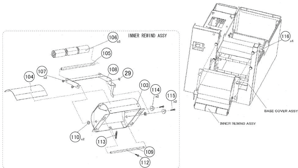
Figure PL6, Inner Rewind Assembly
