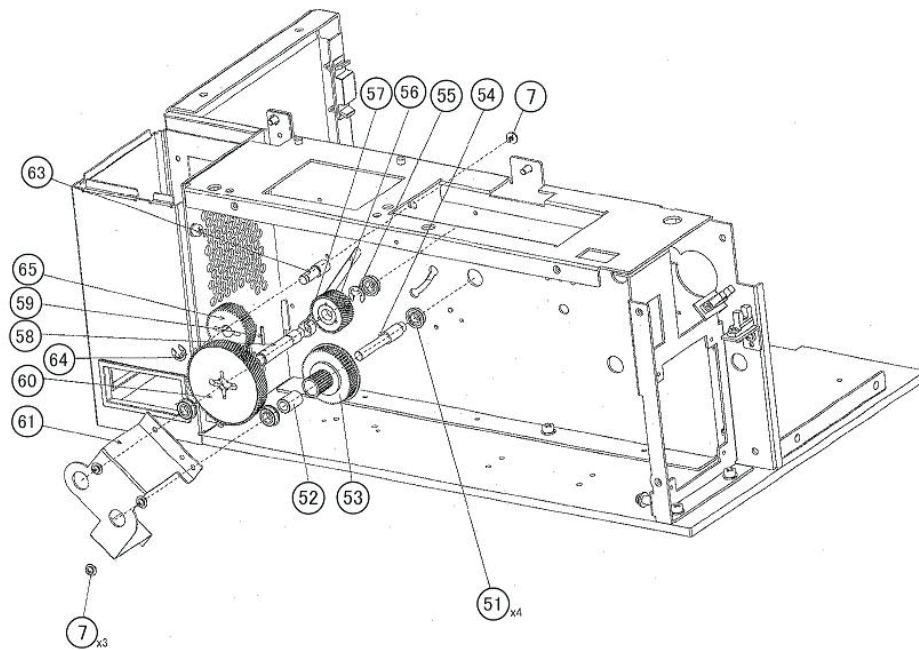
Figure PL3, Gear Pulley Assembly
