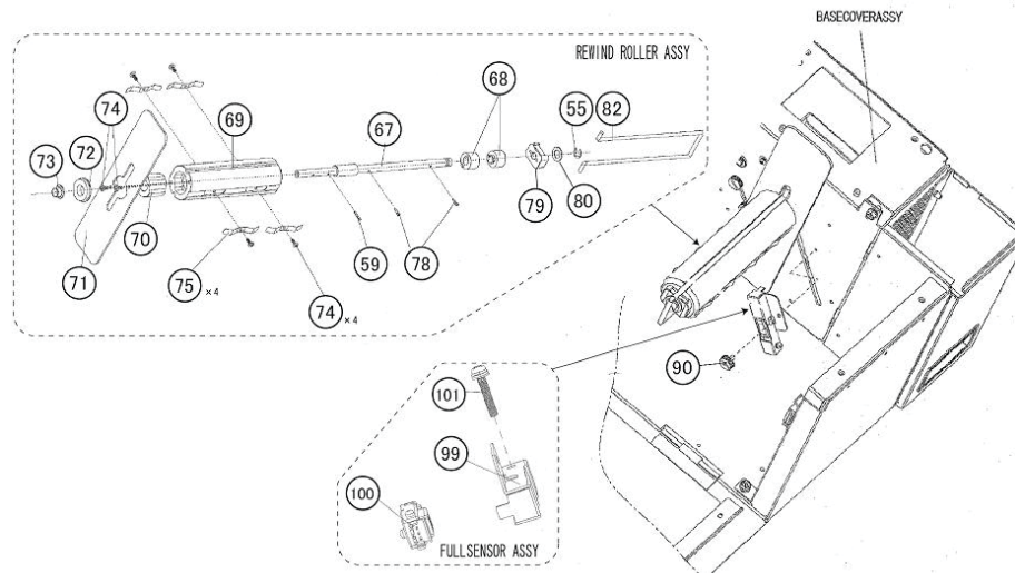
Figure PL5, Full Sensor Assembly
