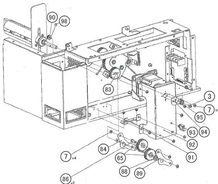
Figure PL4, Rewind Roller Assembly
