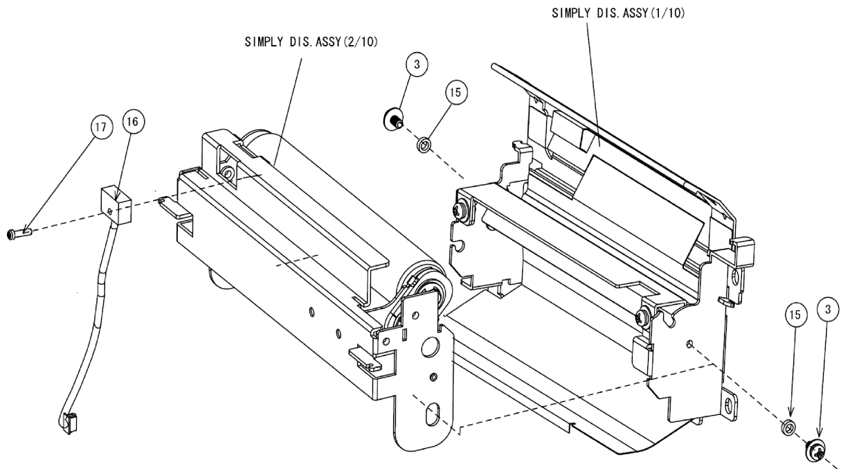
Figure PL35c, Dispenser Assembly
