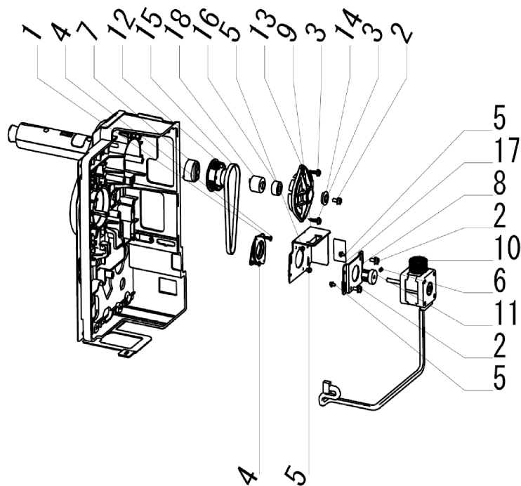
Figure PL30, Ribbon Assembly (3)
