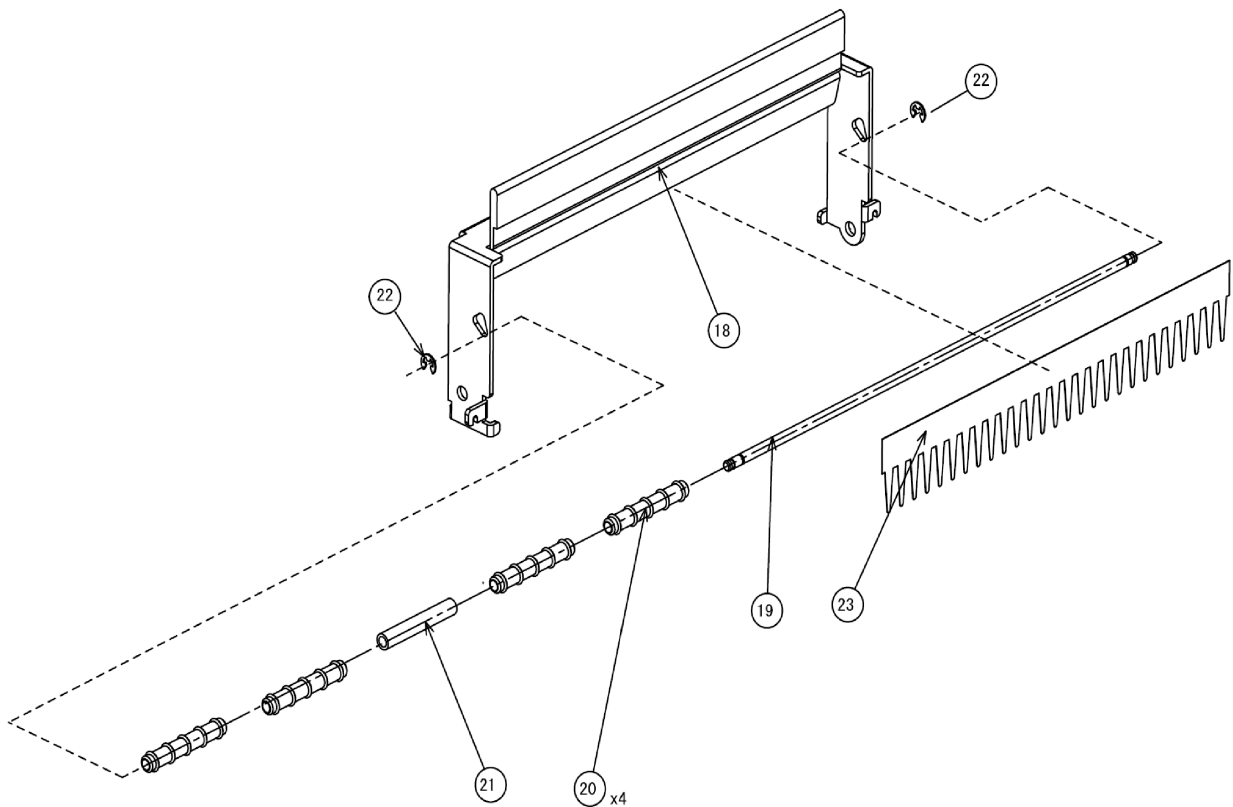
Figure PL35d, Dispenser Assembly
