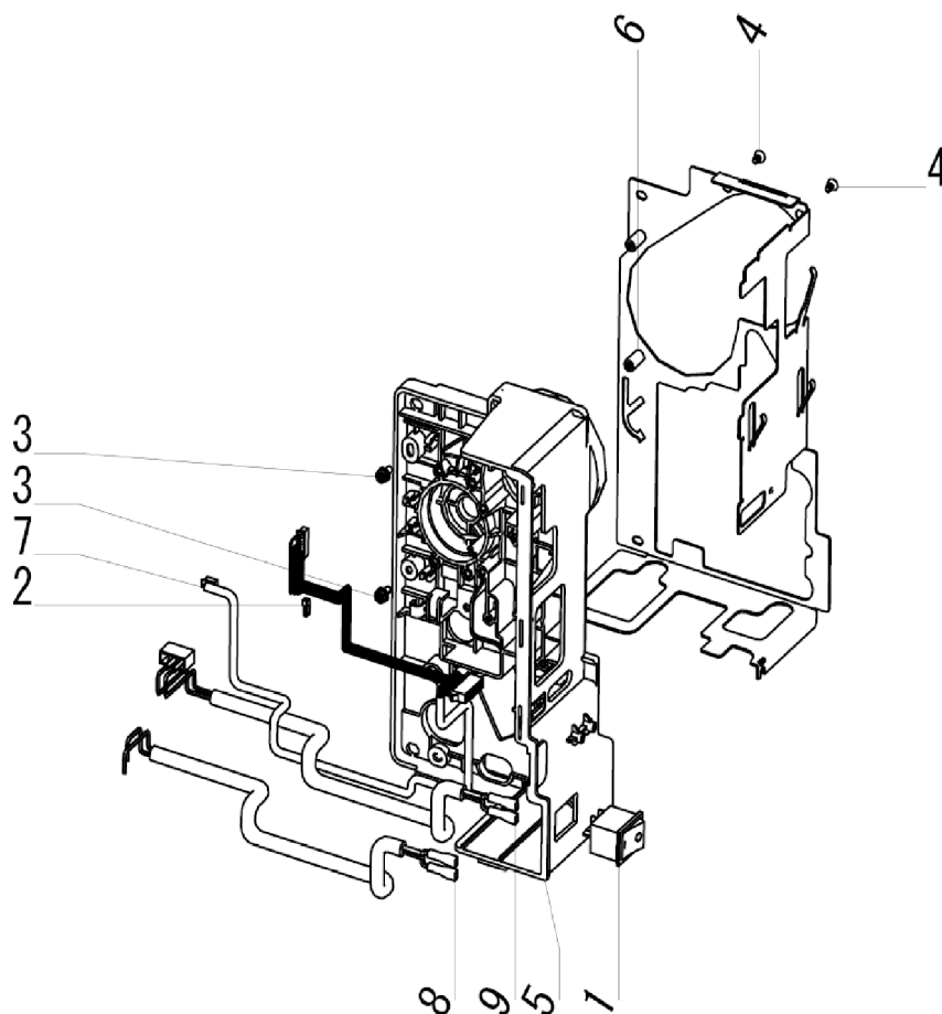
Figure PL7, Frame Assembly (4)
