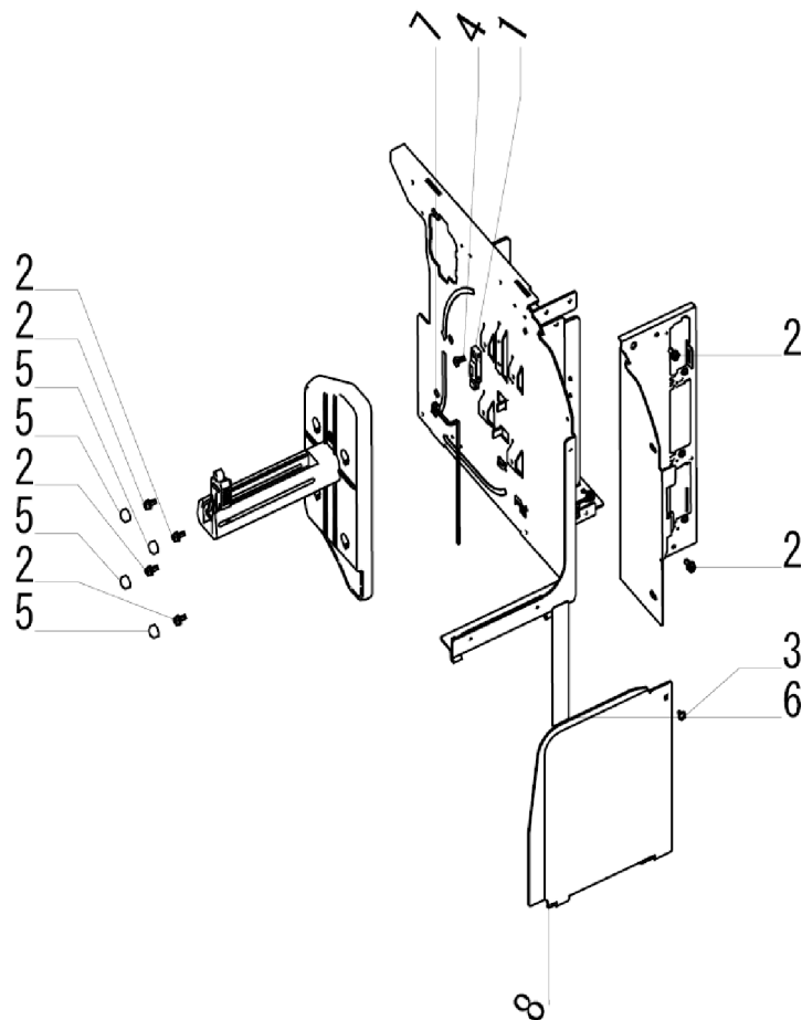
Figure PL9, Frame Assembly (6)
