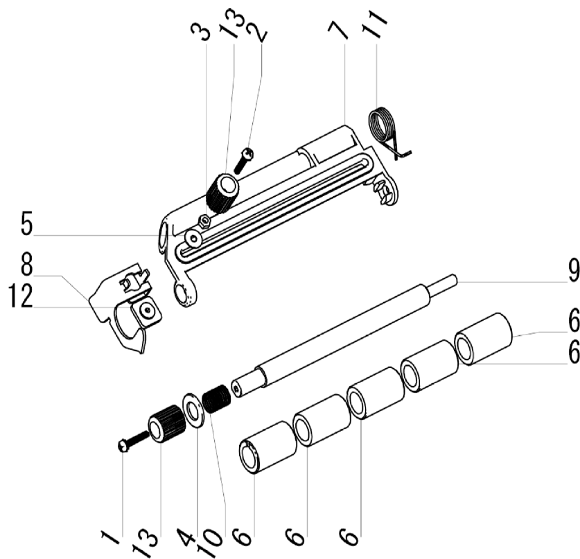
Figure PL20, Print Assembly (4)
