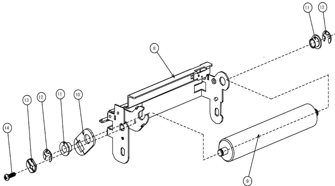
Figure PL35b, Dispenser Assembly (2)
