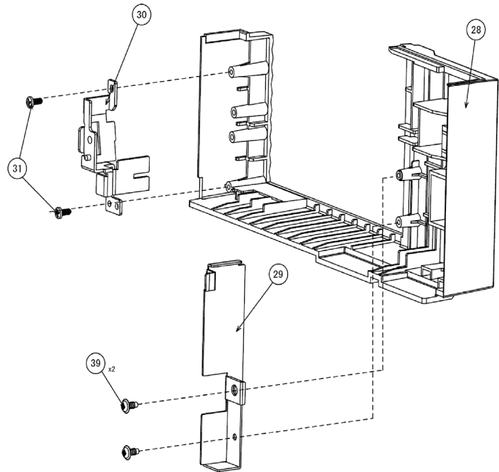
Figure PL35f, Dispenser Assembly
