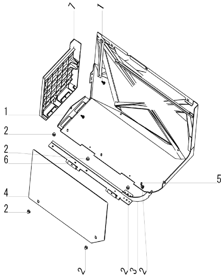
Figure PL2, Housing Cover Assembly (2)
