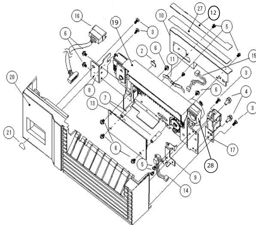
Figure PL33a, Cutter Assembly
