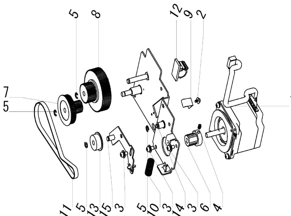
Figure PL16, Drive Train Assembly (3)
