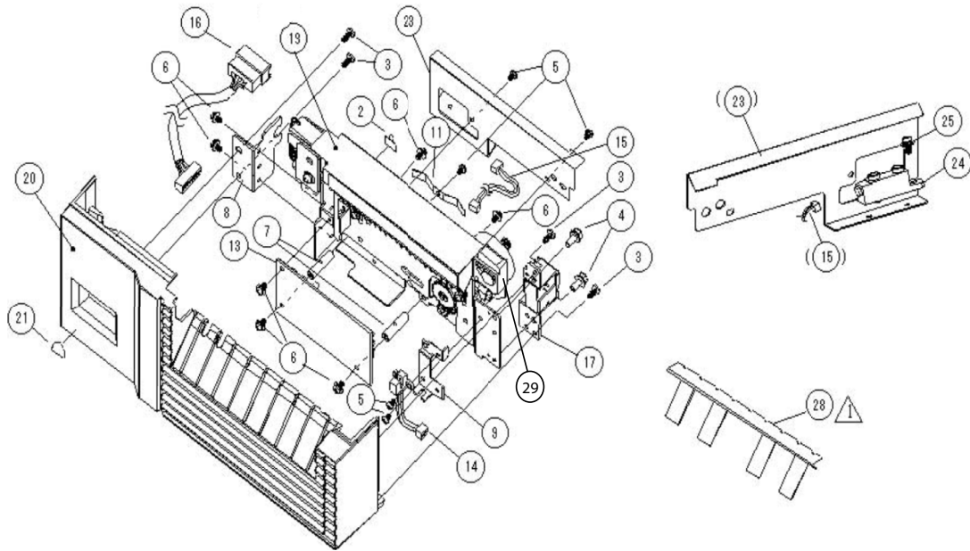
Figure 34a, Linerless Cutter Assembly
