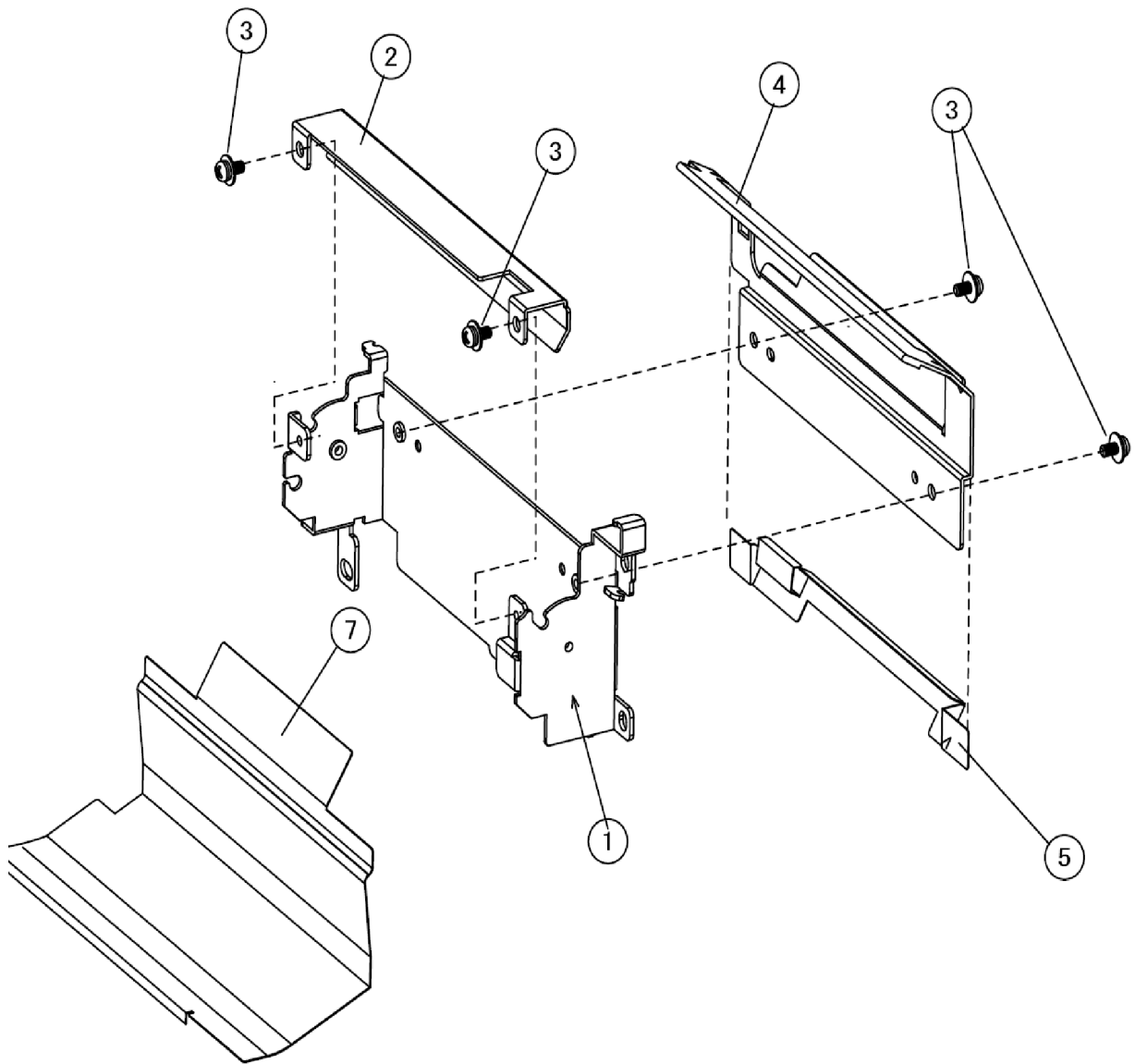
Figure PL35a, Dispenser Assembly (1)
