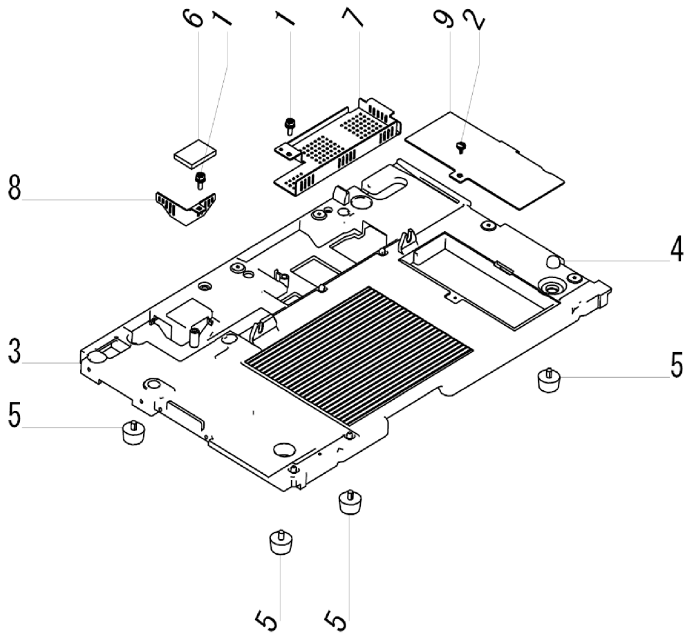
Figure PL13, Frame Assembly (10)
