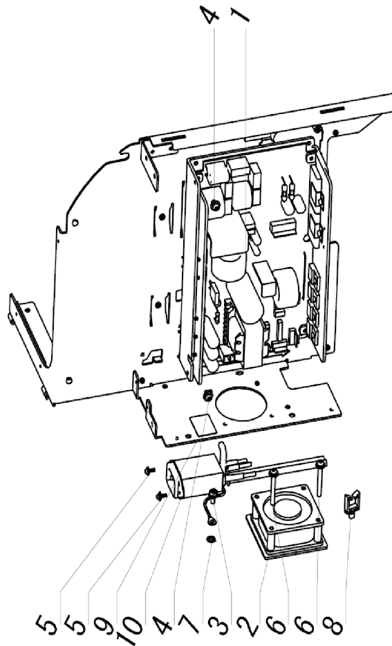
Figure PL10, Frame Assembly (7)
