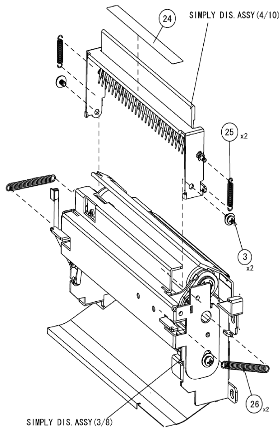
Figure PL35e, Dispenser Assembly
