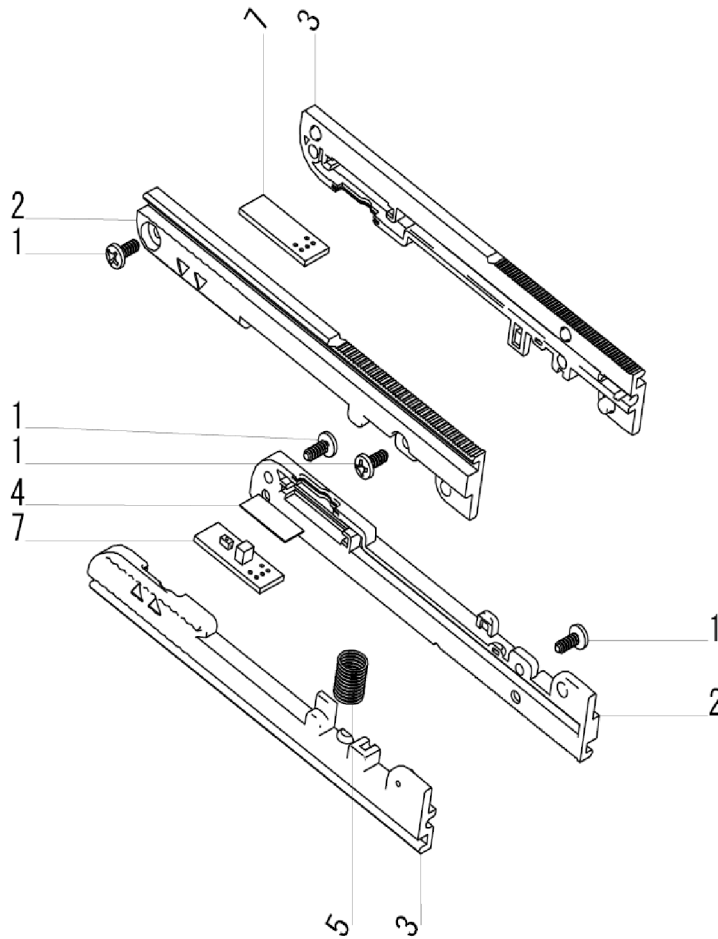
Figure PL21, Print Assembly (5)
