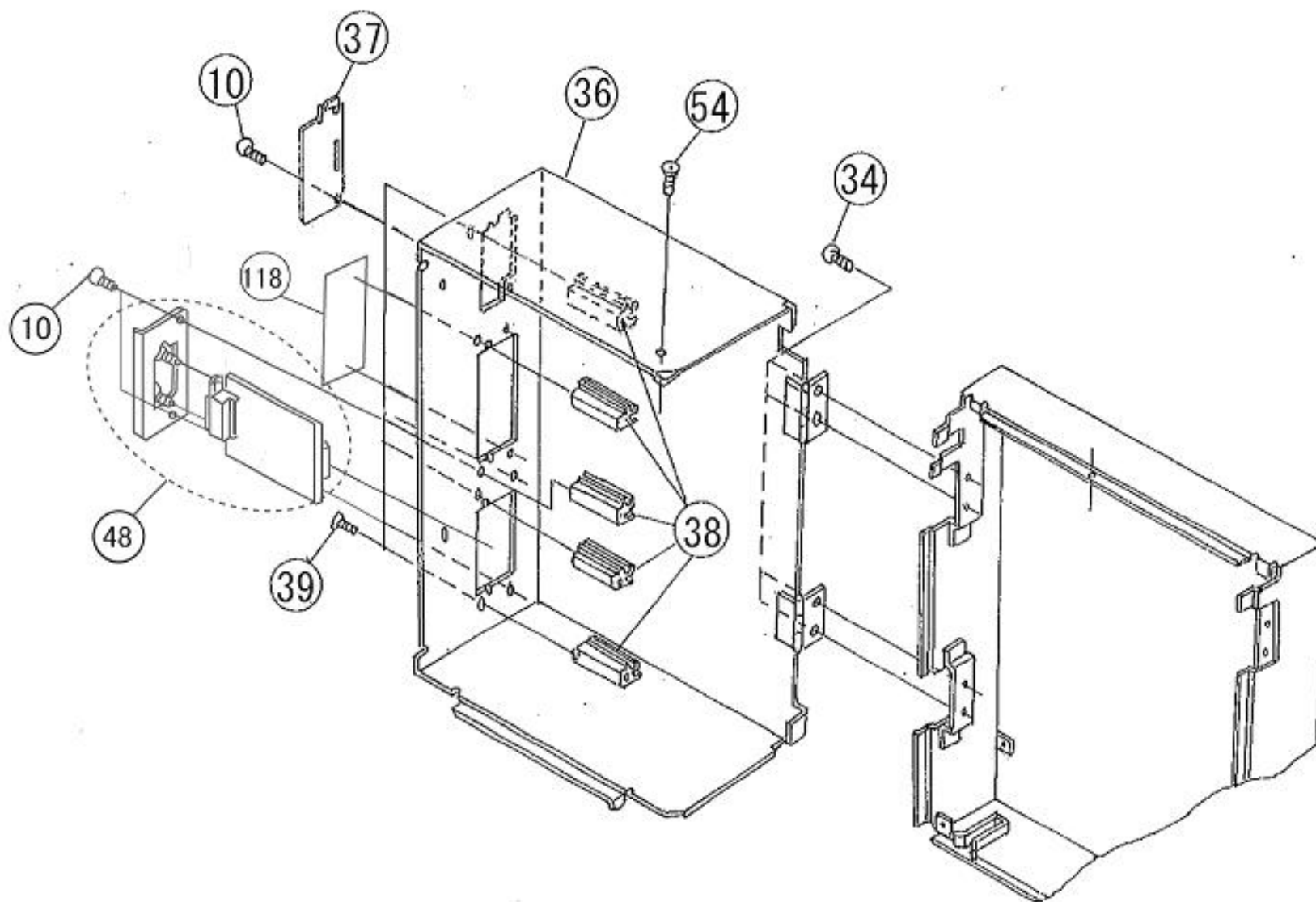
Cover Assembly - 3 Interface Housing
