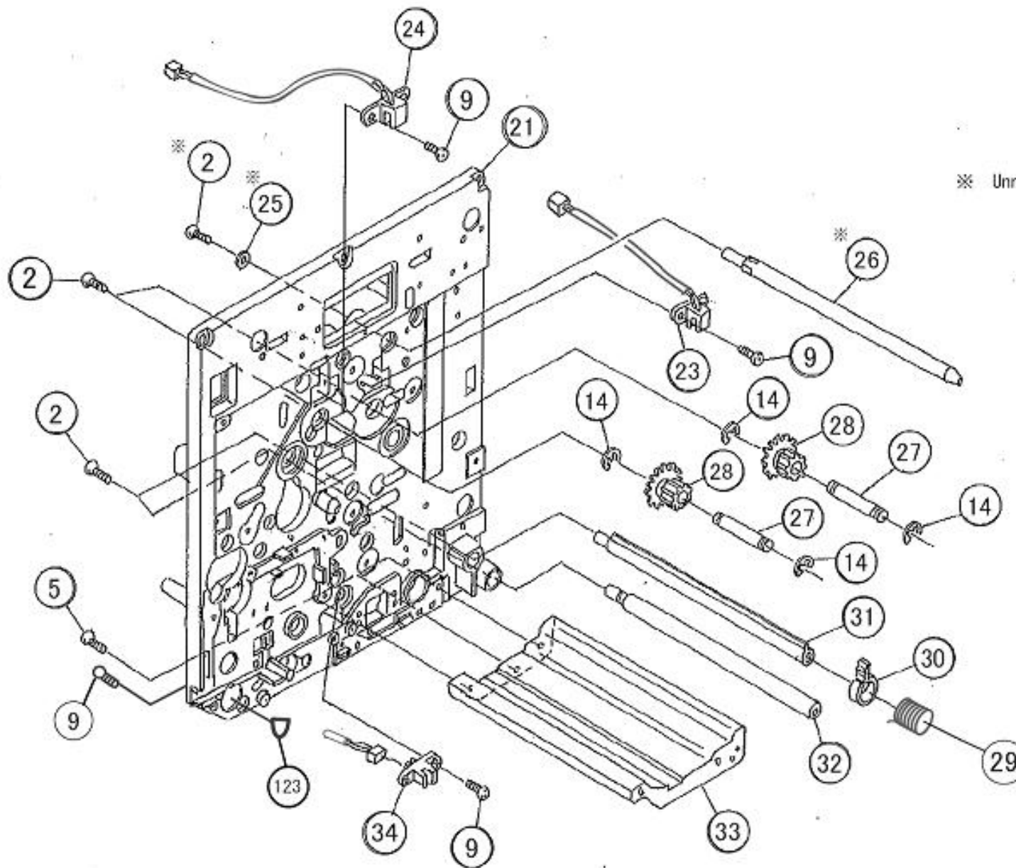
Engine Frame Assembly - 1.1 Main Plate - Front
