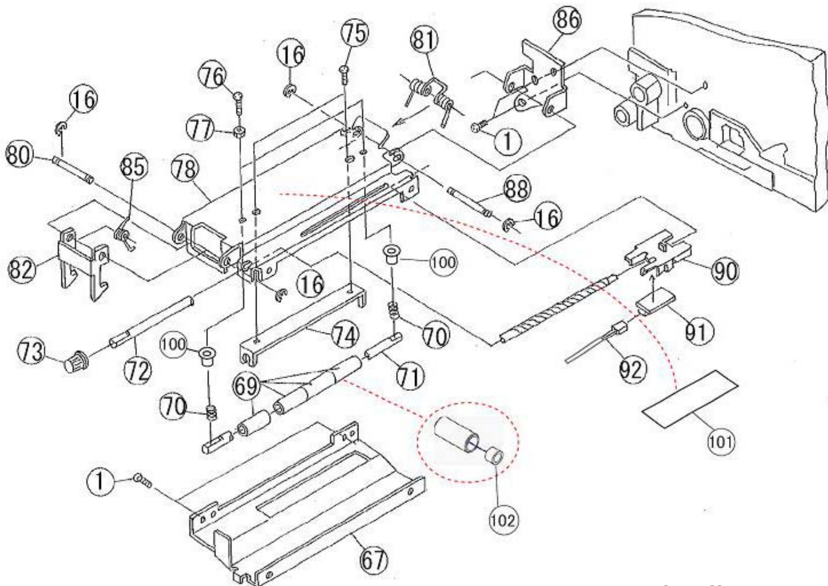
Feed Roller Assembly - 4 Label Sensor
