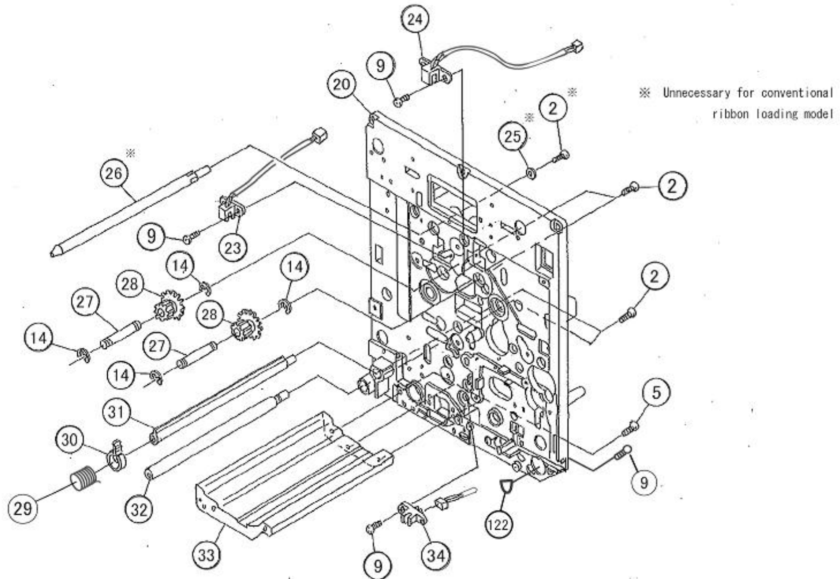
Engine Frame Assembly - 1.1 Main Plate - Front
