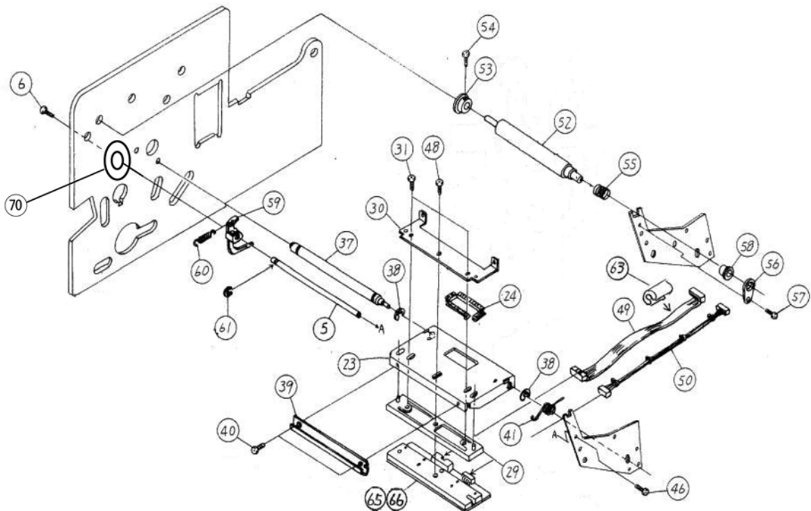
Figure PL3b, Head Assembly
