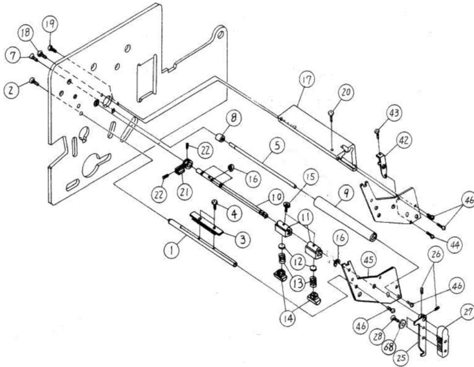
Figure PL3a, Head Assembly
