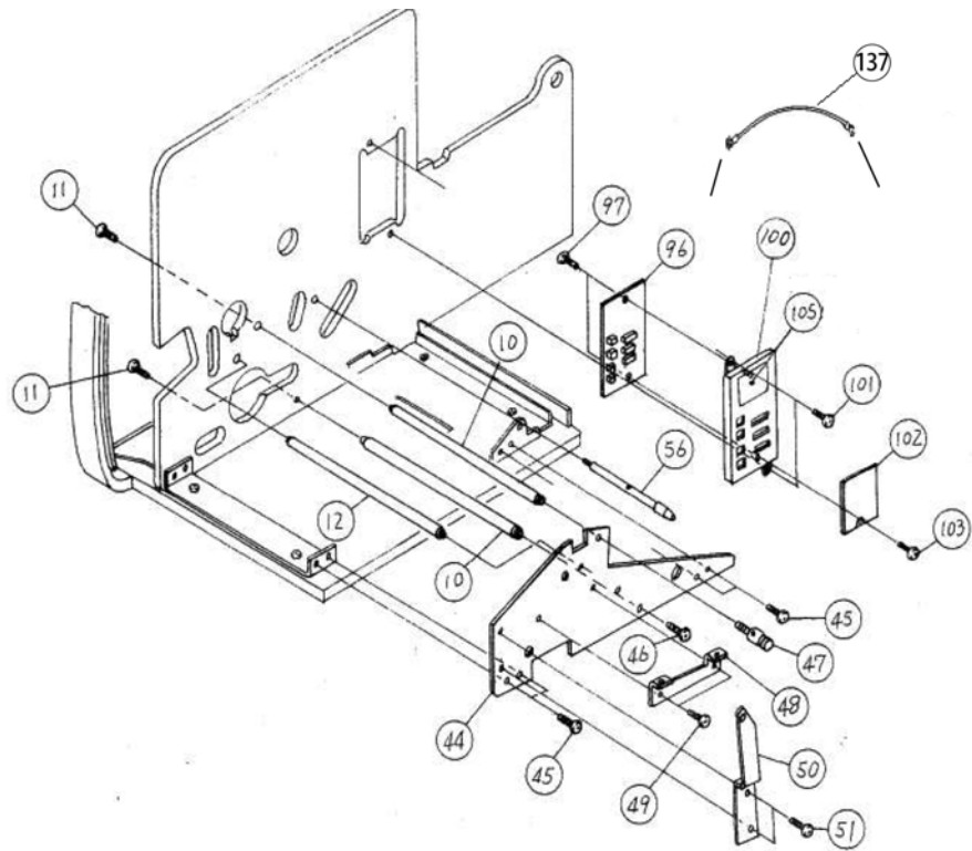
Figure PL1e, Frame Assembly
