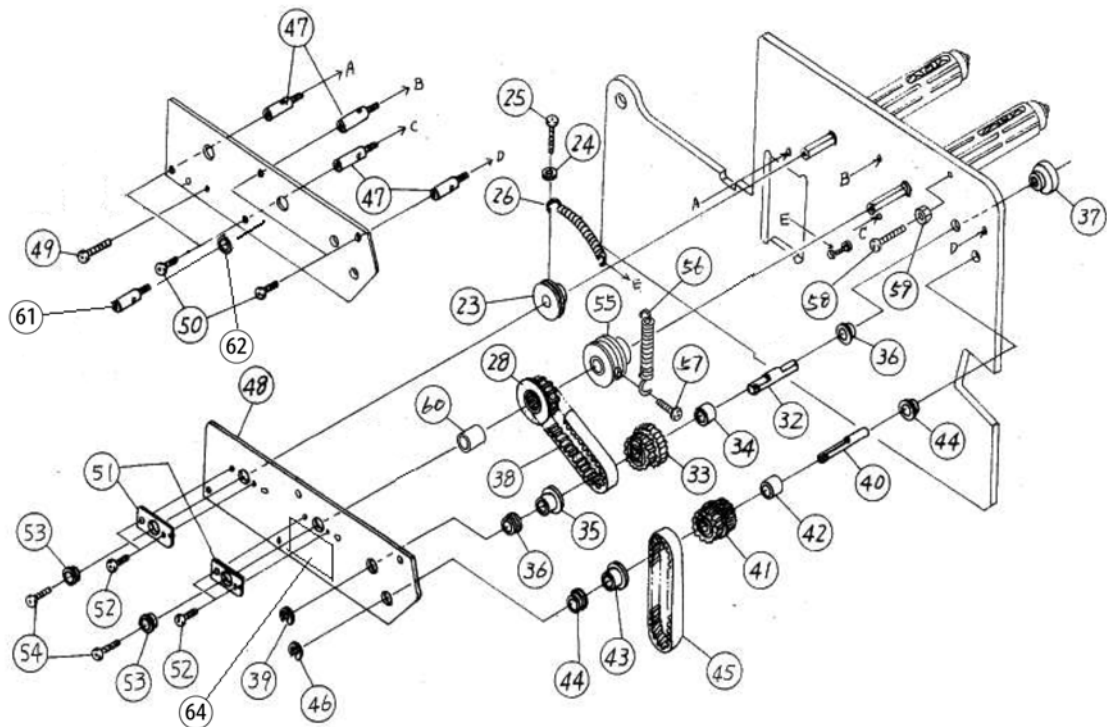
Figure PL4c, Ribbon Assembly
