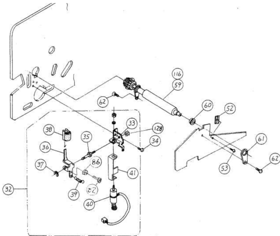
Figure PL1c, Frame Assembly
