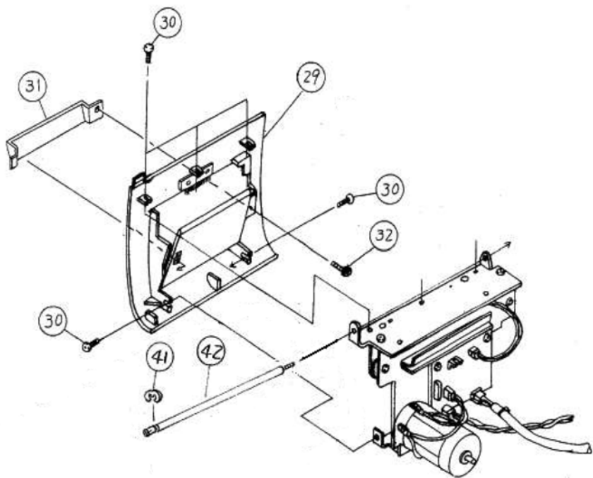
Figure PL9b, Cutter Assembly
