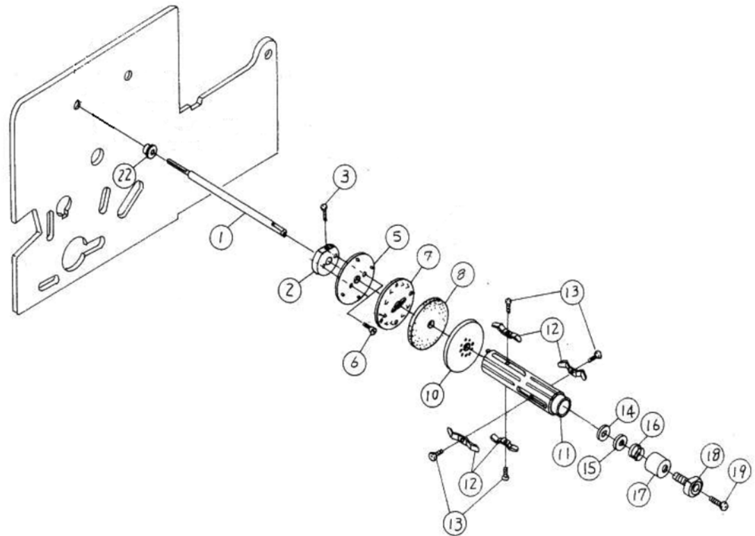
Figure PL4b, Ribbon Assembly
