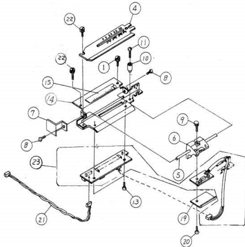
Figure PL8, Cutter Sensor Assembly
