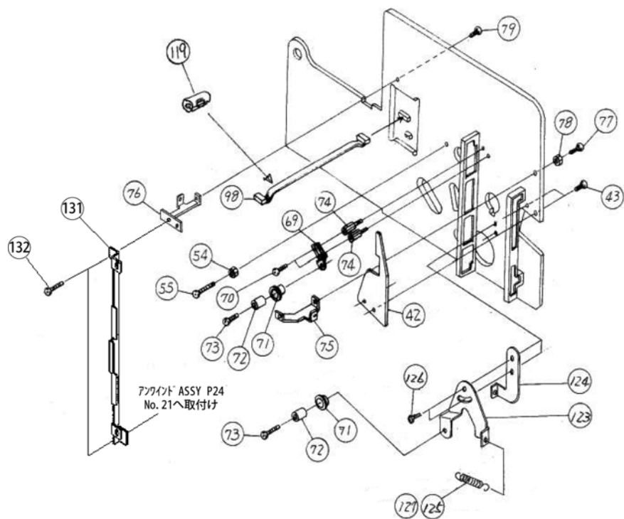
Figure PL1d, Frame Assembly
