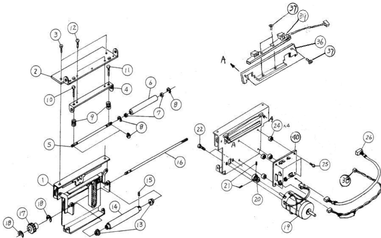
Figure PL9a, Cutter Assembly
