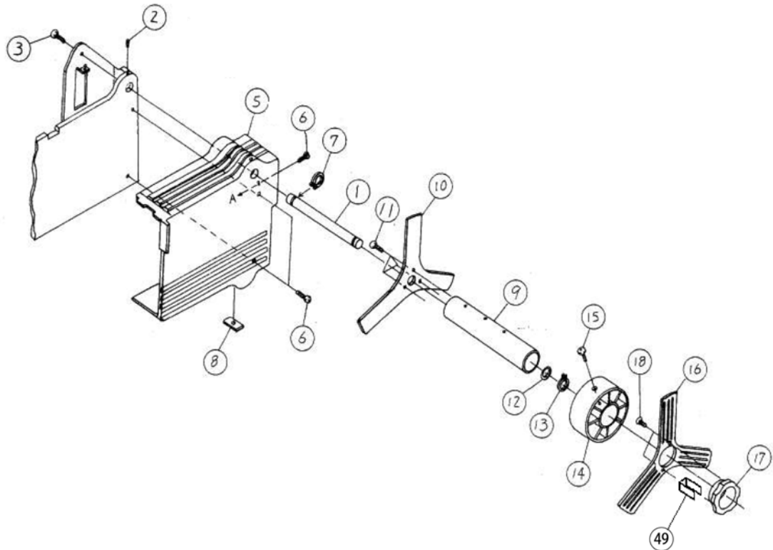
Figure PL5a, Media & Power Supply Assemblies
