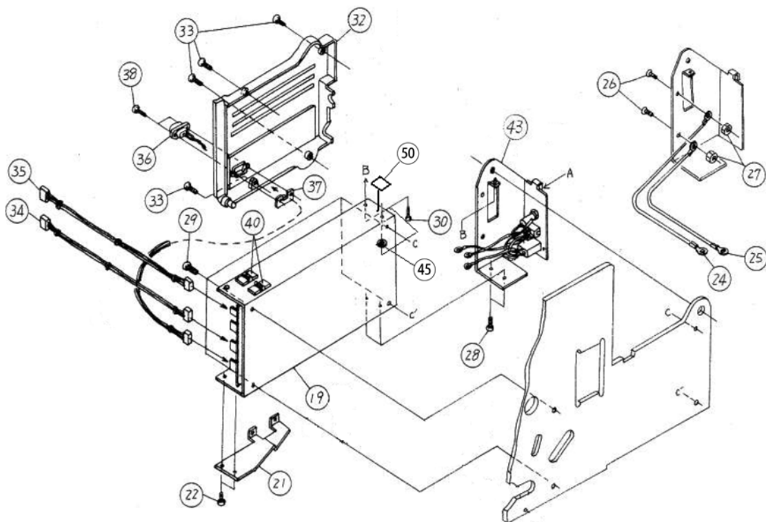
Figure PL5b, Media & Power Supply Assemblies
