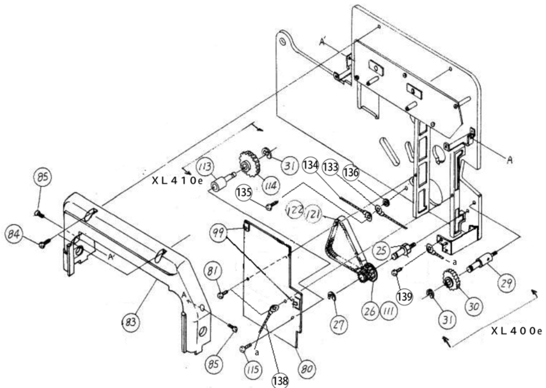
Figure PL1f, Frame Assembly
