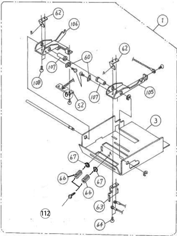
Figure PL2a, Feed Assembly
