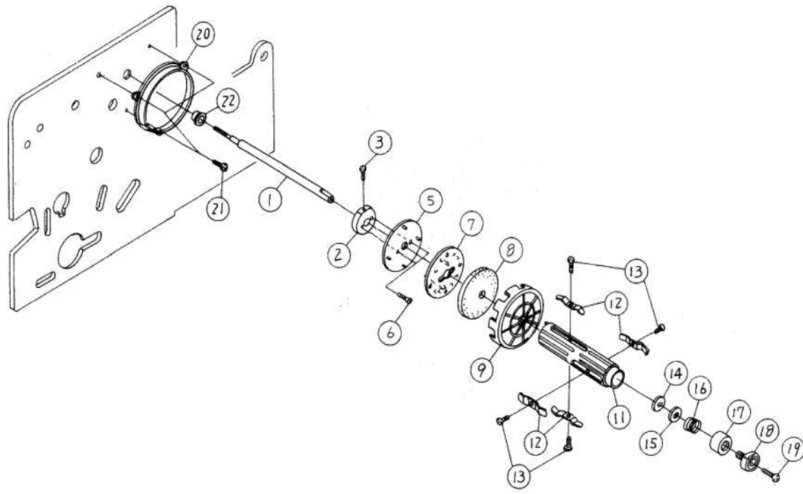
Figure PL4a, Ribbon Assembly
