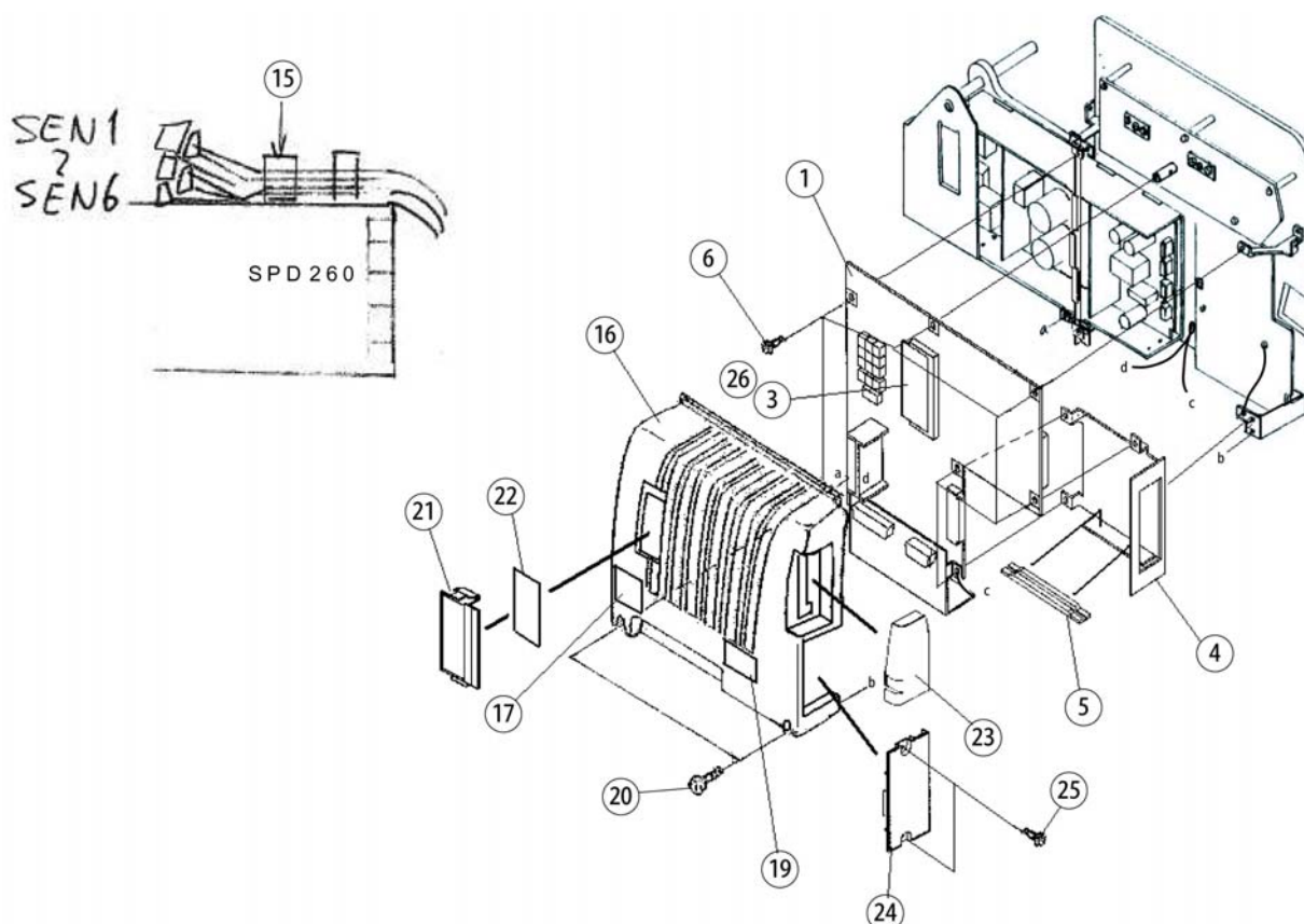
Figure PL7, Rear Cover & Circuit Board Assemblies
