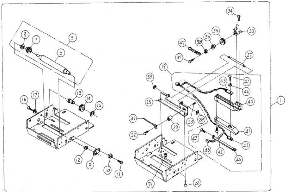
Figure PL2b, Feed Assembly
